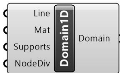
Figure 50 – The Design domain 1D (Domain 1D) component
