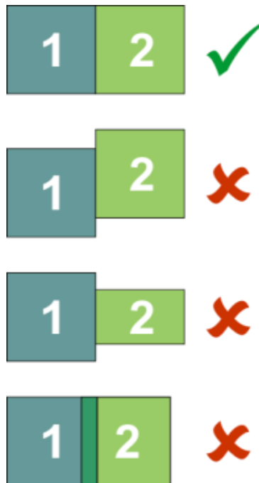
Figure 48 – Allowable mesh interfacing configurations
