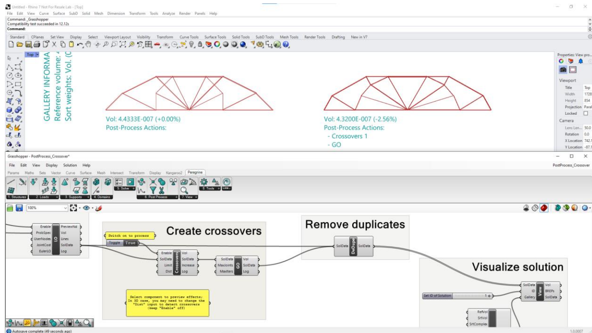
Figure 66 – An example of the output of the crossovers functionality
