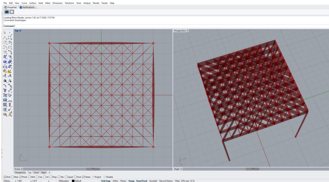
Figure 47 – An example of an optimized grillage structure (supported on four columns)
