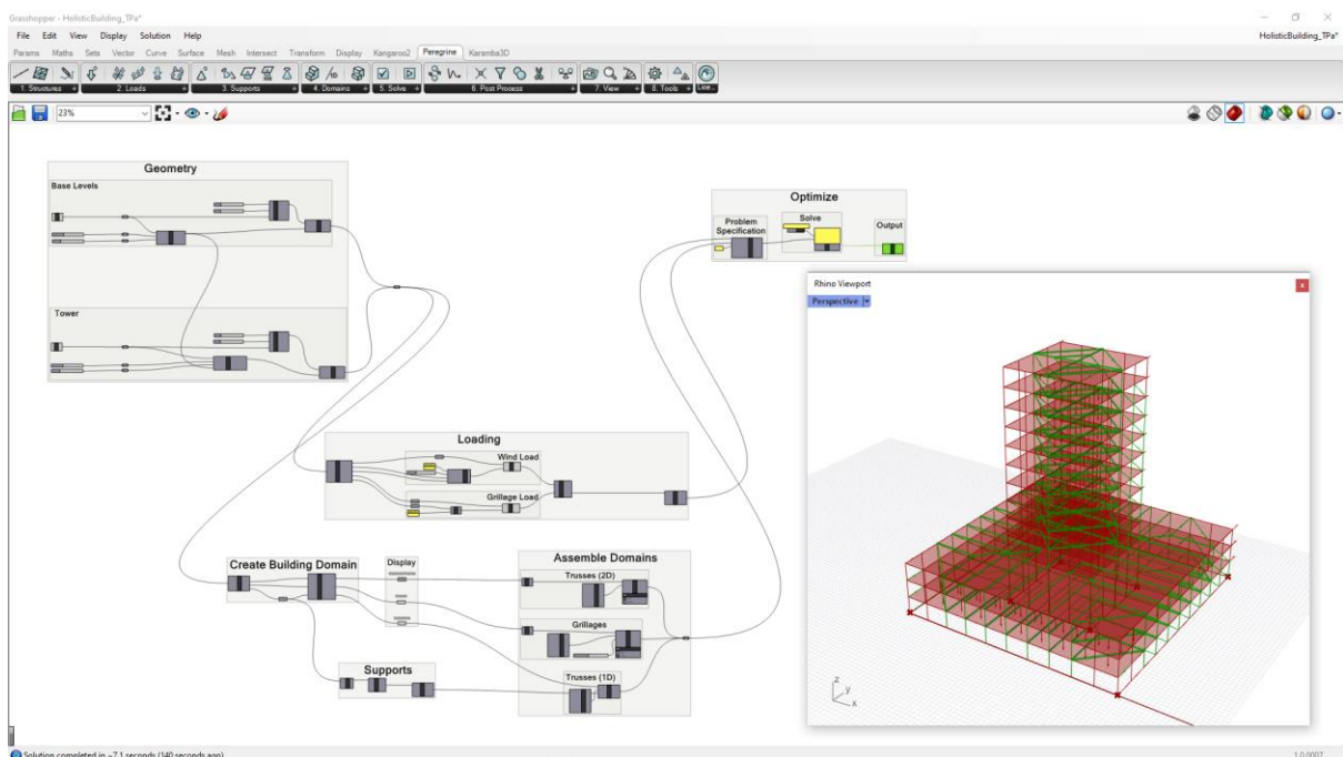
Figure 14 – Optimization of a complex building (grillages and column sizing)
