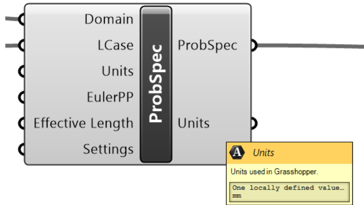
Figure 15 – The unit system can be defined or queried in the ProbSpec component
