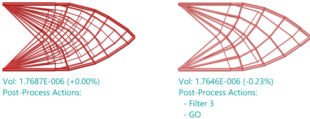
Figure 69 – Filtering the output from Layout Optimization stage (L = original, R = filtered)
