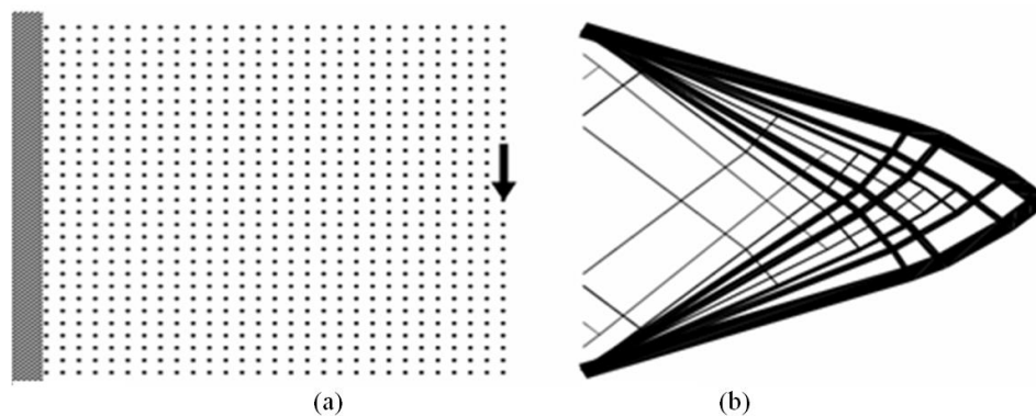
Figure 92 – Example layout optimization
