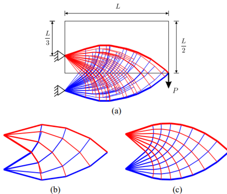
Figure 93 – Rationalization of a cantilever truss (a) by using joint cost and GO (b) and GO (c)
