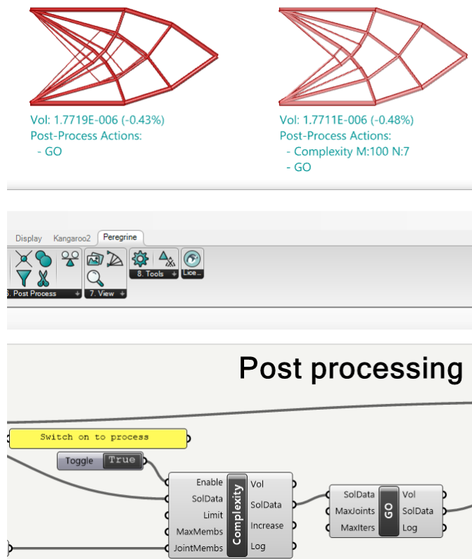
Figure 75 - Reducing the complexity of the solution (left = original, right = refined)
