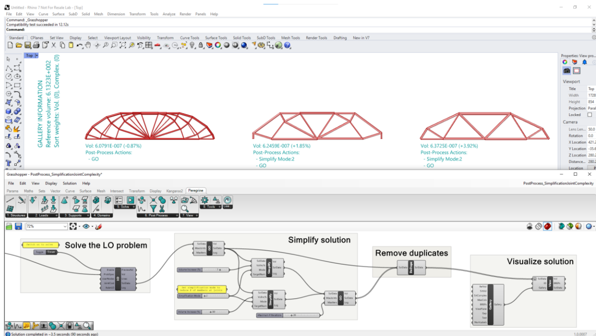
Figure 63 – Simplification of a truss structure
