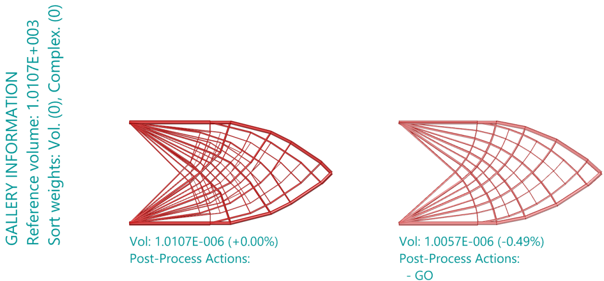
Figure 60 - The GO component used to reduce the complexity of a solution
