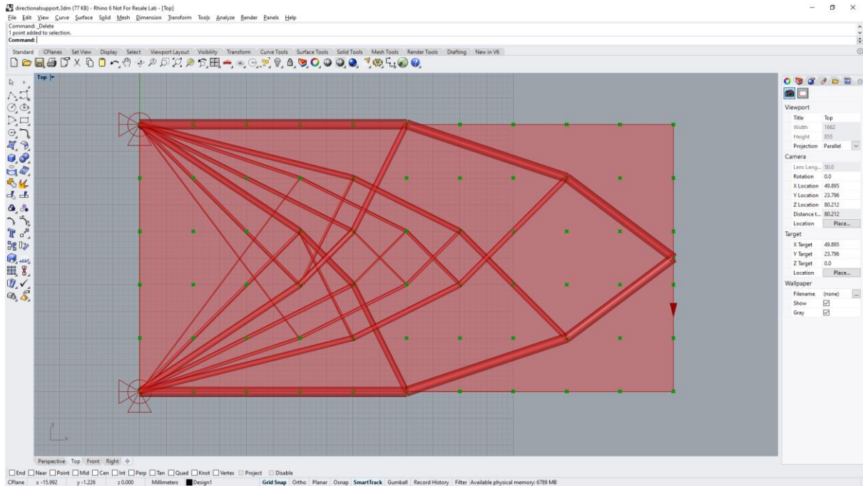
Figure 57 – The Simple2D problem in Rhino. Nodes previewed in green
