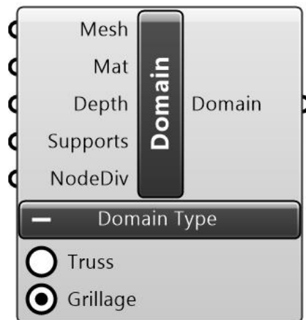
Figure 45 - The Design Domain (Domain) component - Grillage
