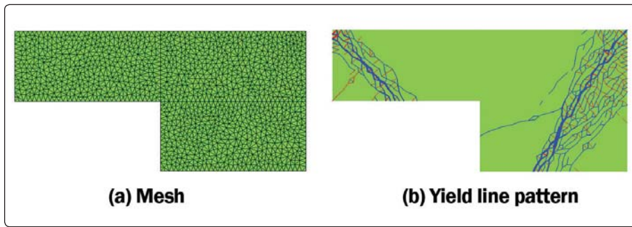
Figure 3: Results from the 2011 research ( \lambda=5.47 ).
