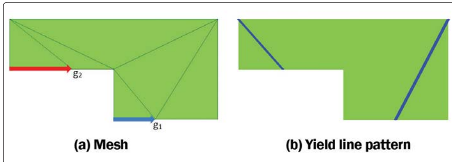
Figure 4: Results for a coarse unstructured mesh from EFE ( \lambda=4.38 ).
