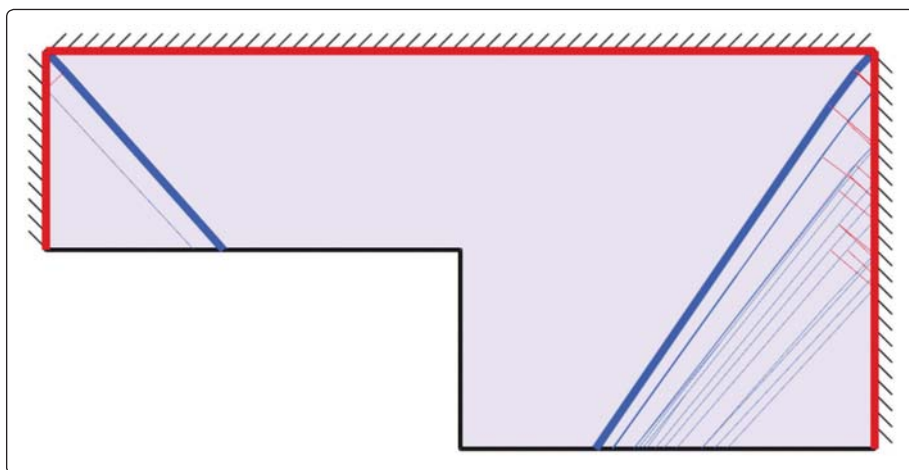
Figure 5: DLO solution of 2014 using 4000 nodes ( \lambda=4.21 ).
