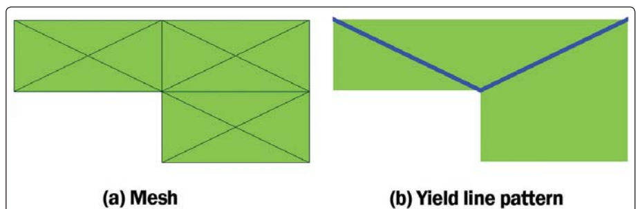
Figure 2: Results from the 1997 research ( \lambda=5.86 ).
